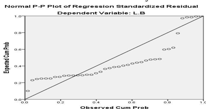
Gambar 1 Grafik Normalitas Probability Plot
